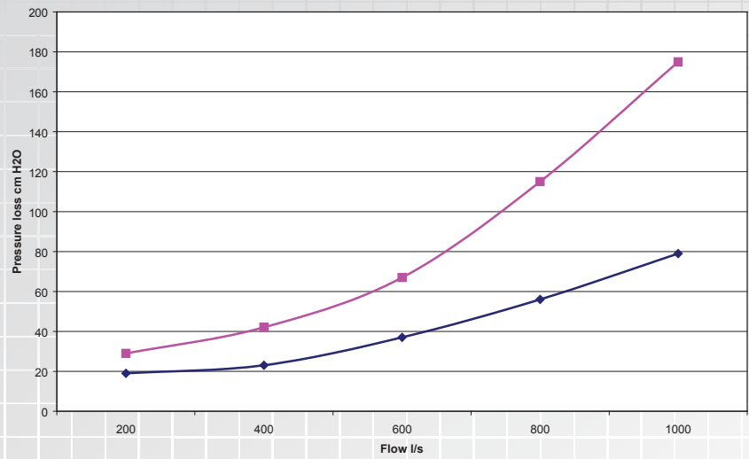
AVK Ball Check Valve DN500
