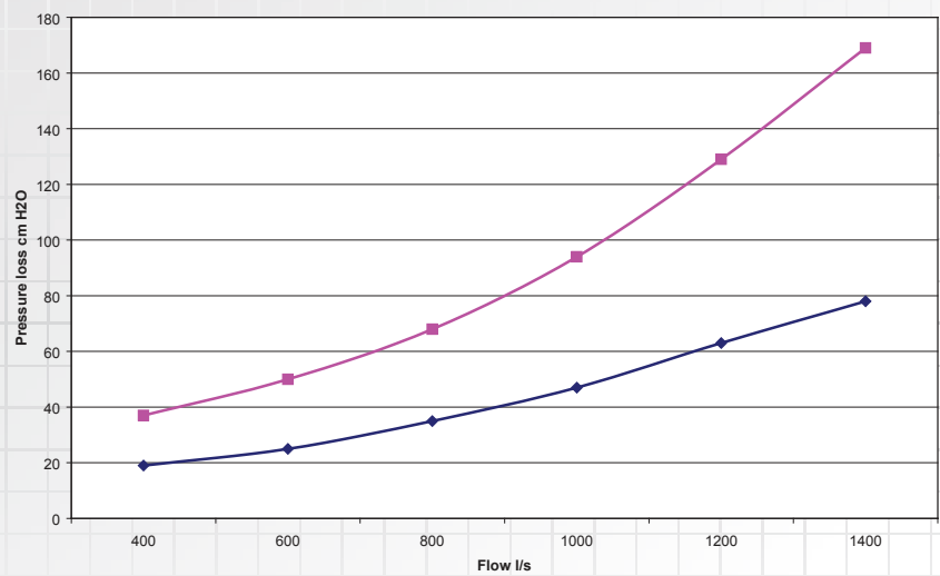
AVK Ball Check Valve DN600
