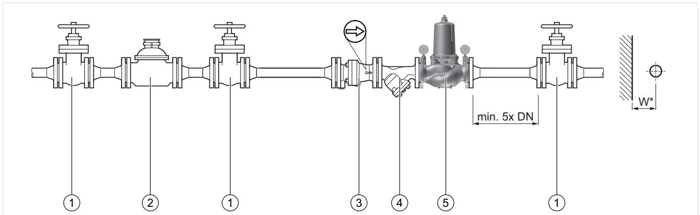
Fig. 1 Standard installation example for the pressure reducing valve
