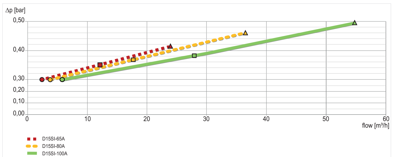
Fig. 2 Pressure drop within the valve in dependency of the flow rate and the used connection size (Sizes DN65 - DN100)
